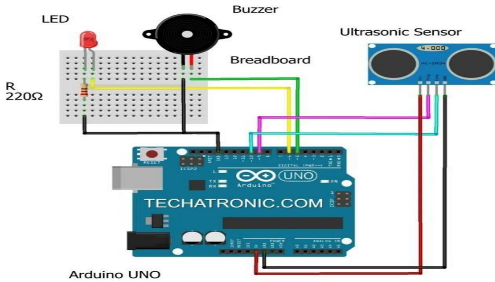
Block Diagram of Smart Blind Stick Using Arduino Uno and Sensor
