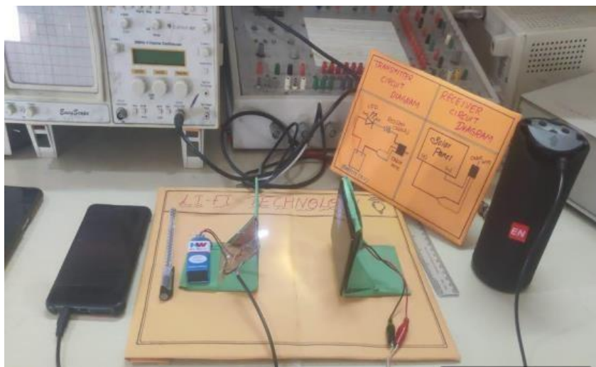
Fig 2: Experimental Setup
