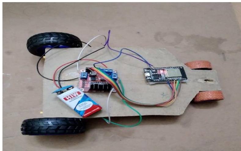
Fig b: Experimental Setup
