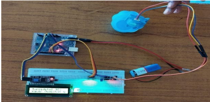
Fig 2: Experimental Setup
