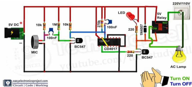
Fig 1: Circuit Diagram of Automatic home control system using sound Technology
