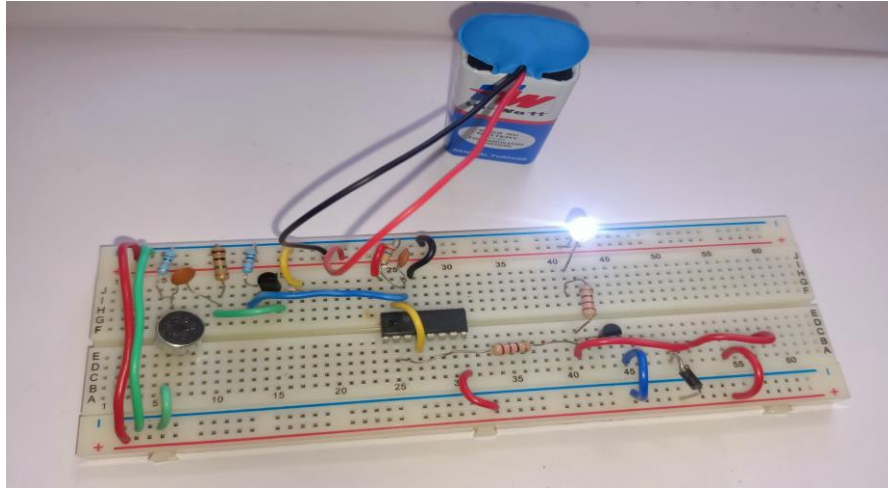
Fig 2: Experimental Setup
